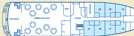
Frangipani Deck
